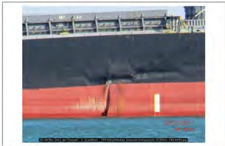
28-30 Mar 2011 Jpn Tsunami - C. Scawthorn - 759 Fukushimaken Imaizumi Komagamine 37.8551; 140.9499
