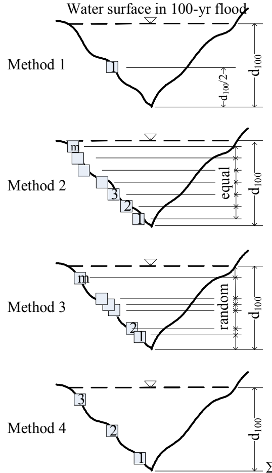
Figure G-2. Four methods of simulating X
